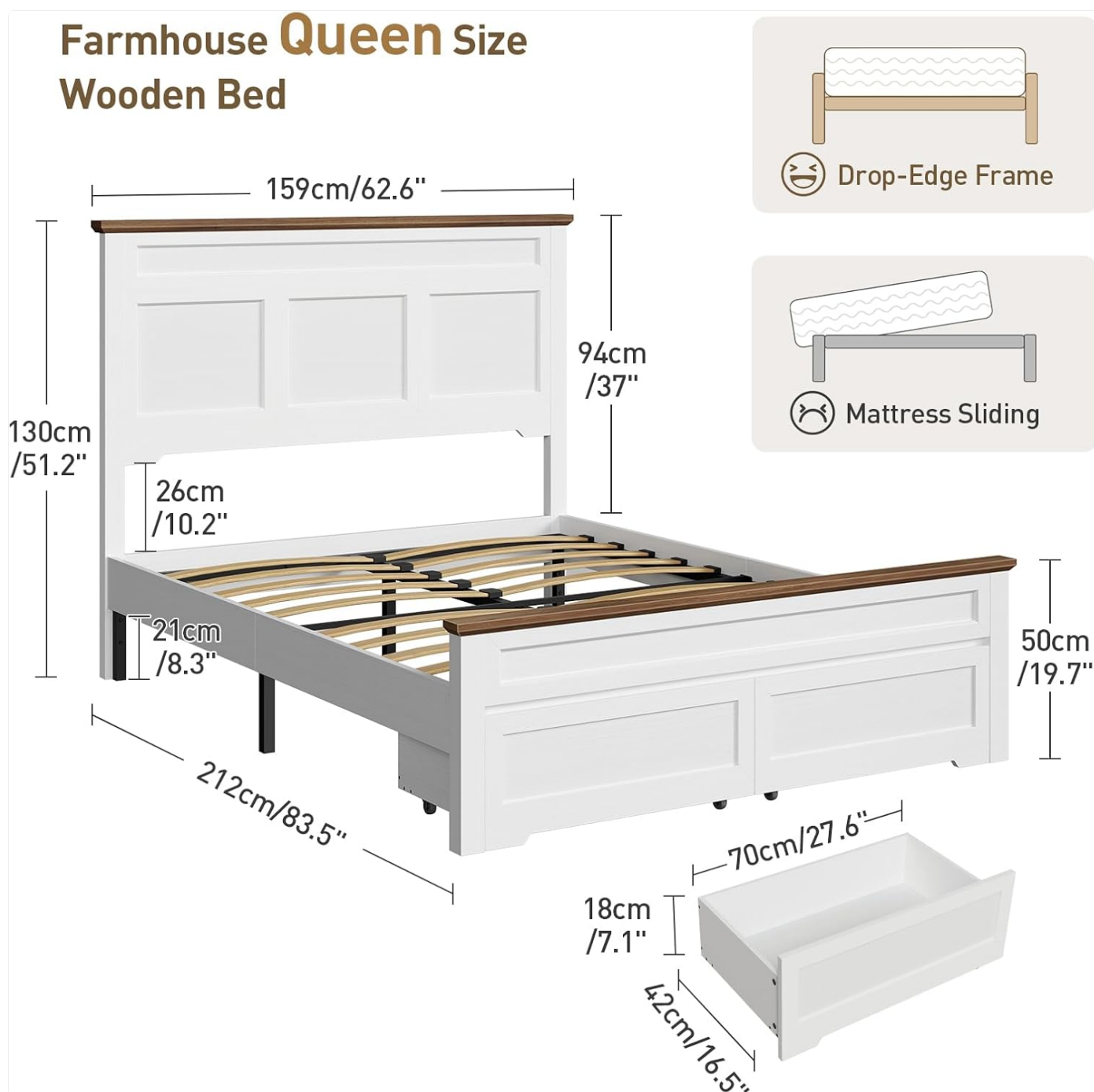
Image 3.1: An illustrative diagram showing the overall dimensions of the queen size bed frame, including the headboard, footboard, and storage drawers, along with key features like the drop-edge frame and slat system.
