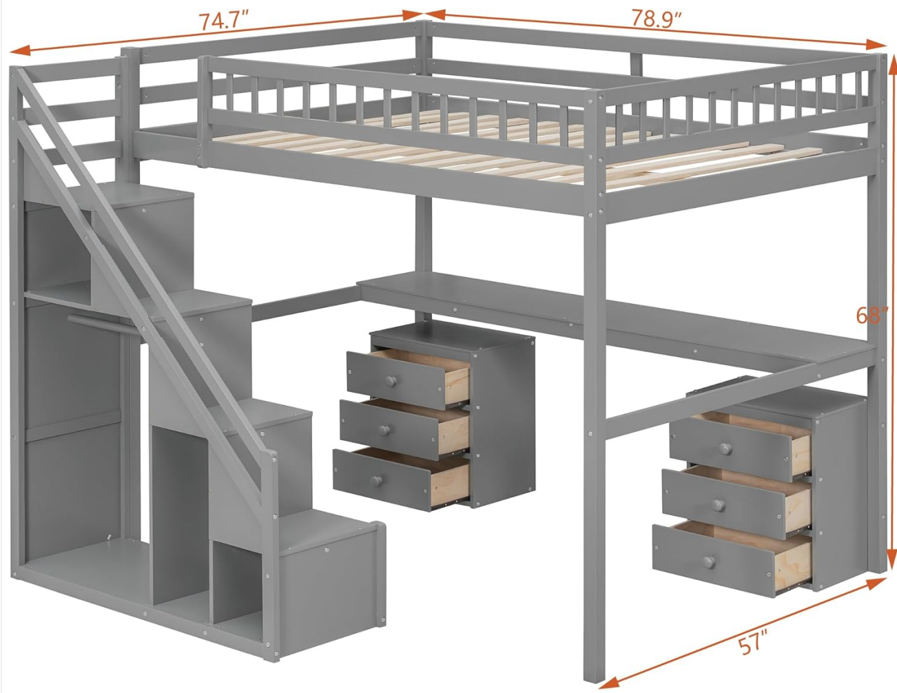
Detailed diagram showing the dimensions of the Bellemave Full Loft Bed: 78.9 inches (L) x 74.7 inches (W) x 68 inches (H).
