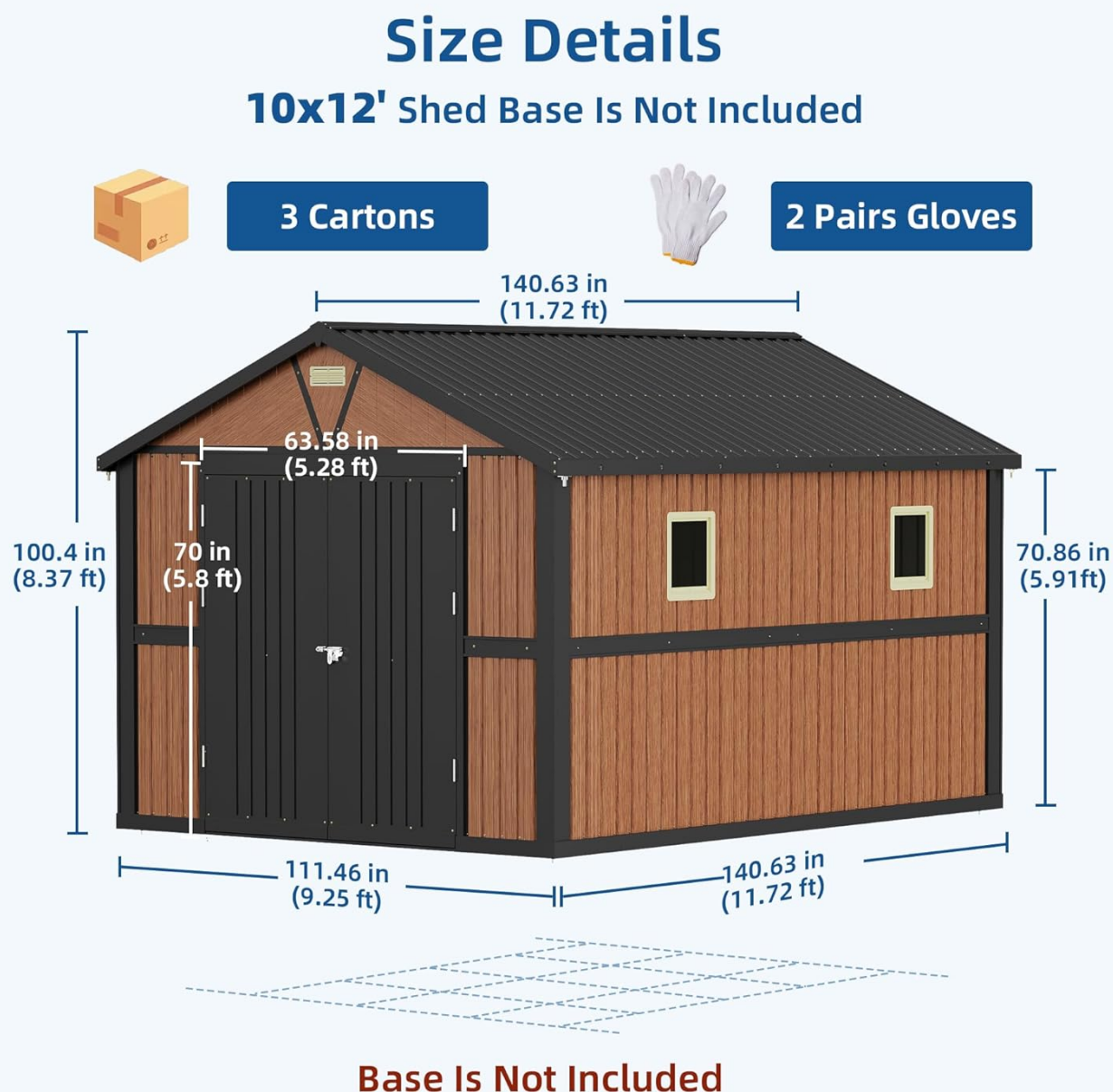
Image 3.1: Overview of shed dimensions and package contents.
