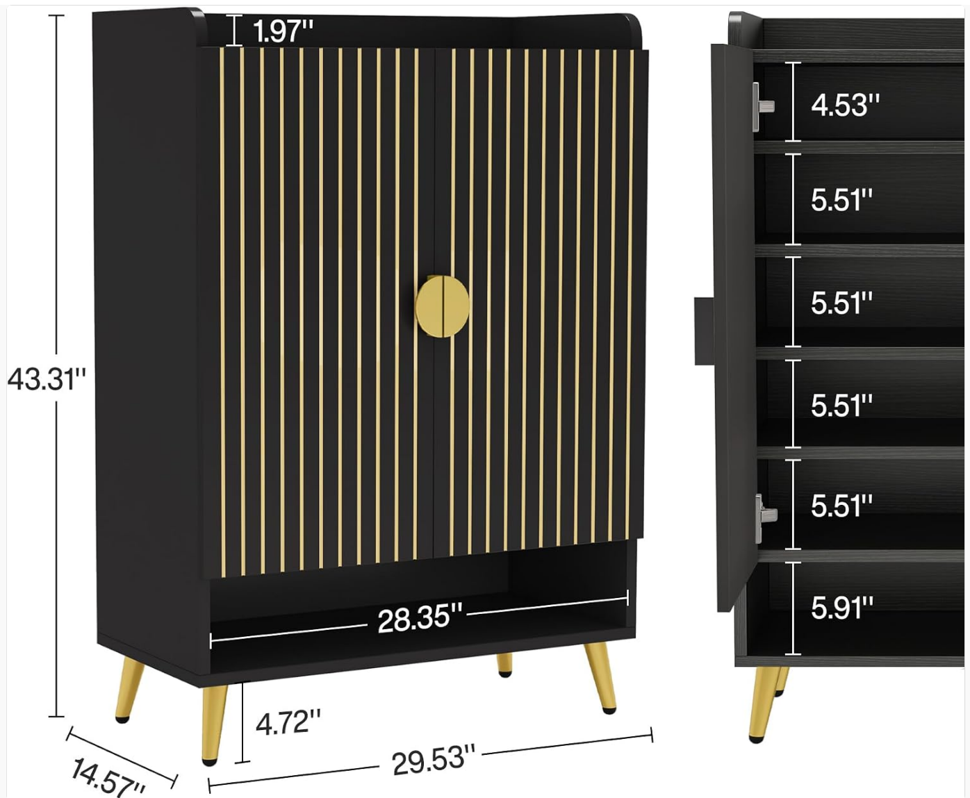
Figure 3.1: Detailed dimensions of the shoe cabinet, including height, width, depth, and internal shelf spacing.
