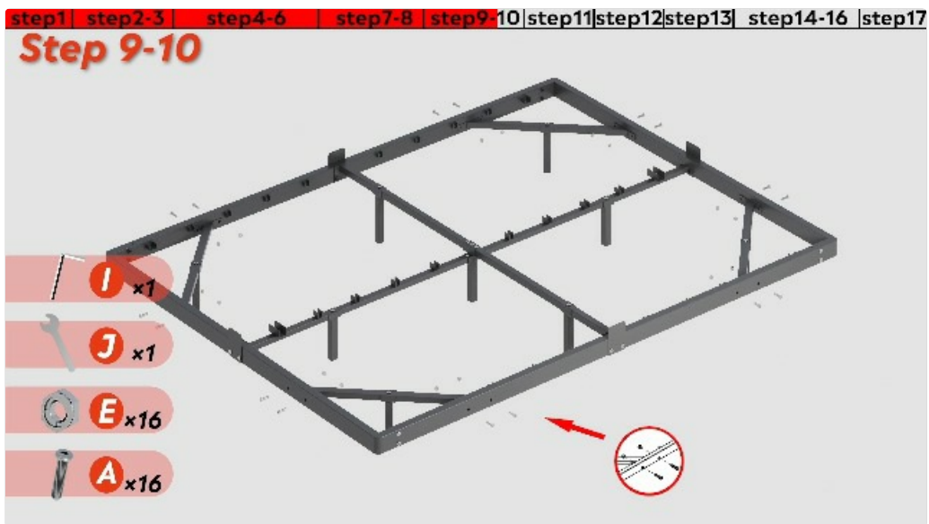
Figure 1: Assembly Instructions Diagram (from video "ACHJ005 006 007 bed frame")
