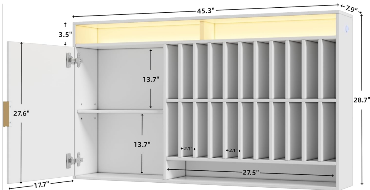
Image 4.1: Product dimensions and internal layout.
