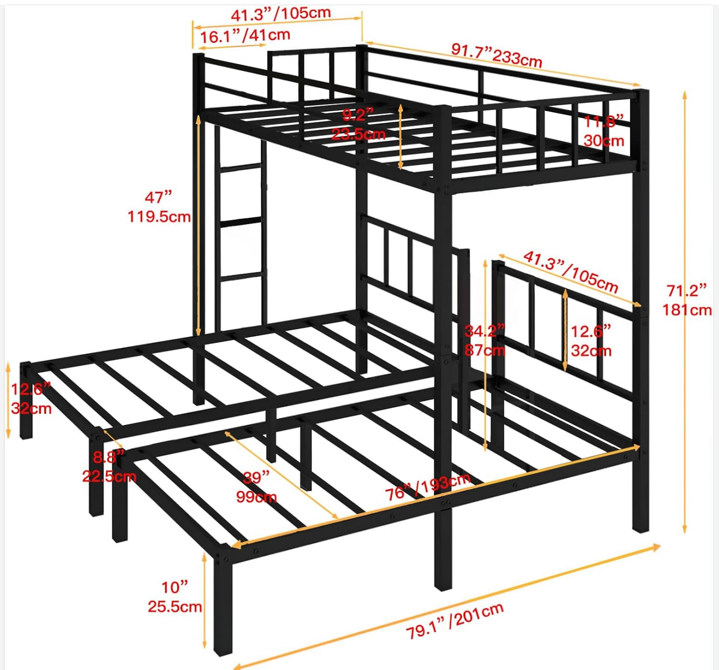
Image: Comprehensive dimensions of the bunk bed, including height, length, and width for each section.
