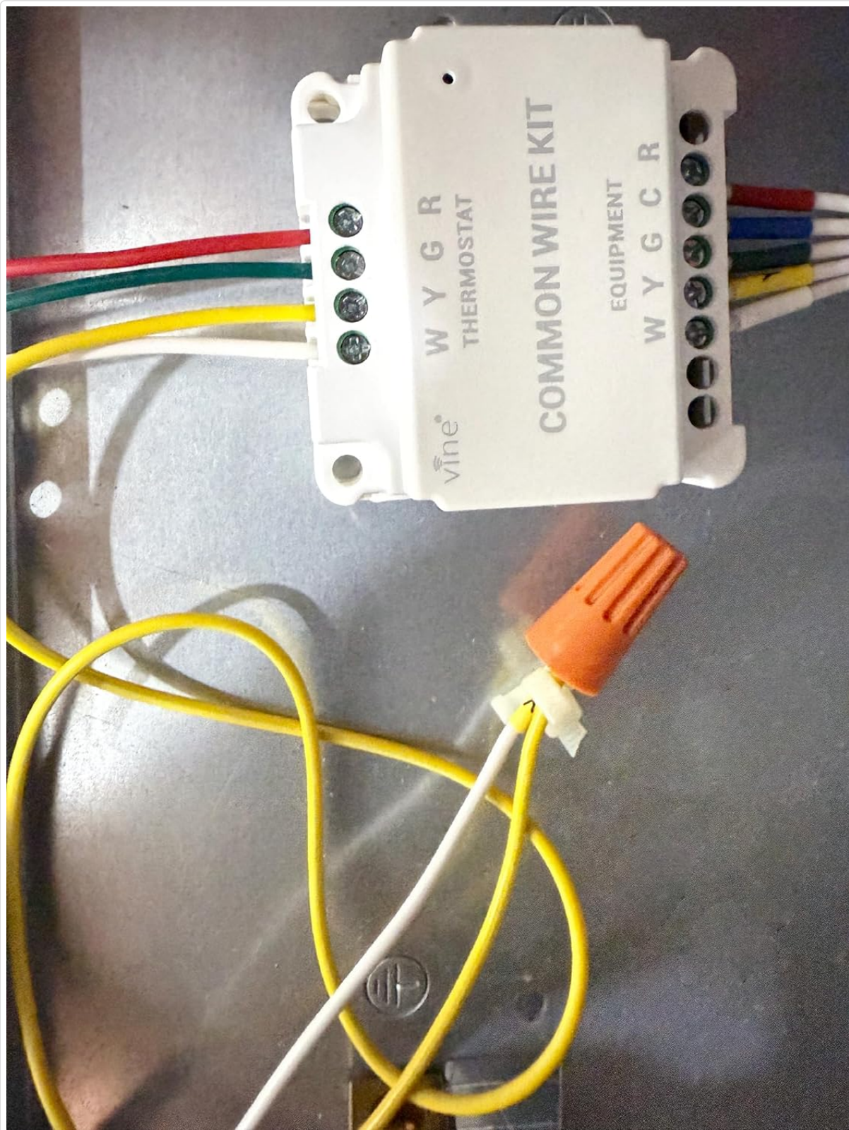
Image: C-Wire Adapter Connections at Control Board. A close-up view of the Vine C-Wire Adapter connected to an HVAC control board. Wires from the adapter are neatly connected to the board's terminals, and a wire nut is used to secure a connection, demonstrating proper wiring technique.
