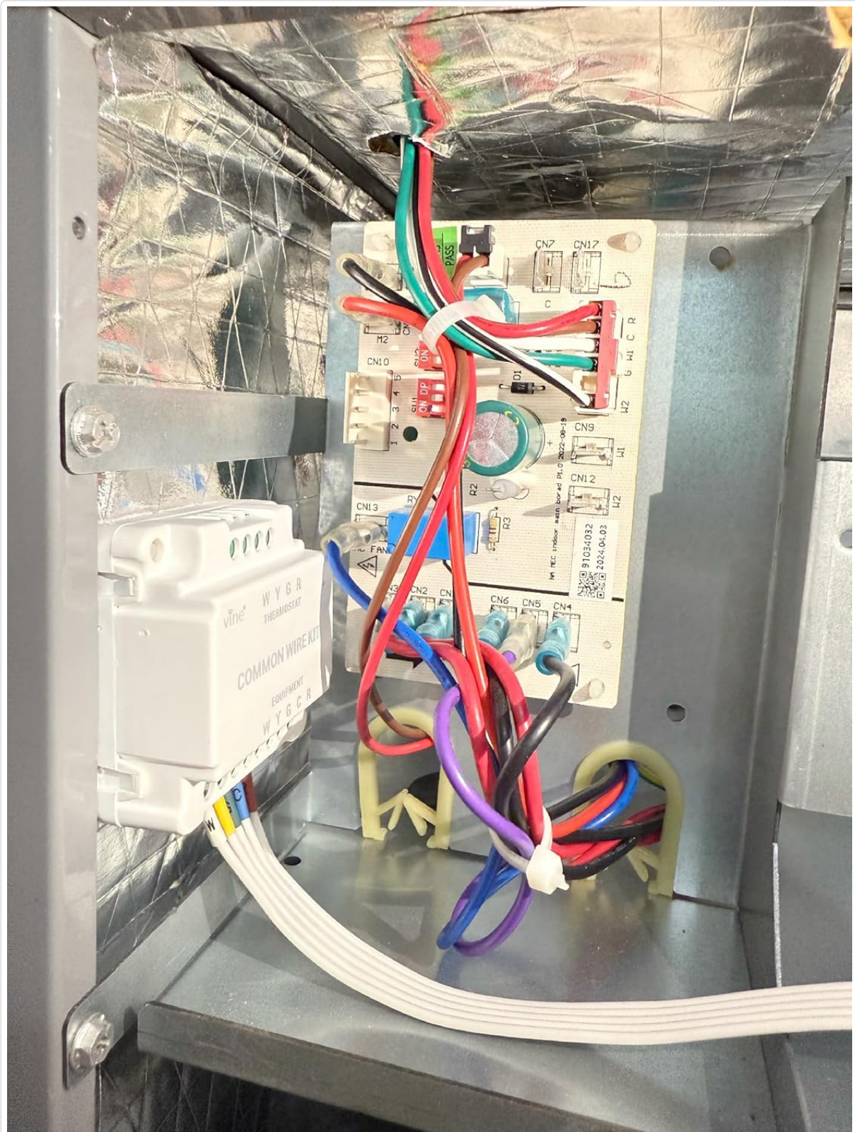
Image: C-Wire Adapter Installed in HVAC Unit. This image shows the Vine C-Wire Adapter unit mounted inside an HVAC system, with its wires connected to the main control board. The adapter is positioned to manage the wiring between the thermostat and the HVAC unit.
