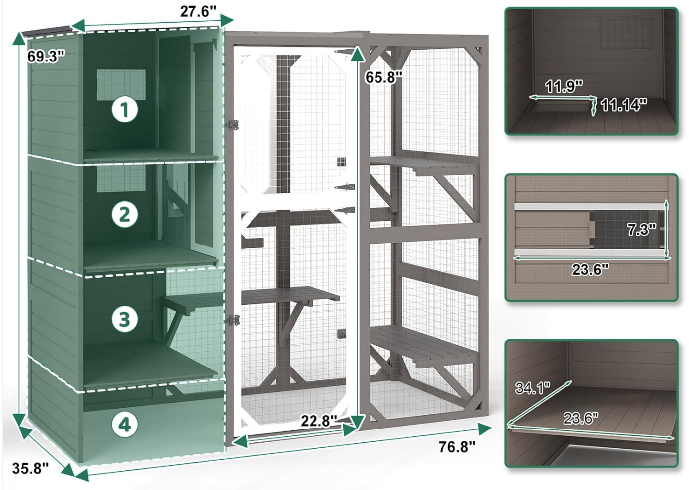
Figure 2: Detailed product information and dimensions, illustrating the two-box delivery and key measurements of the catio components.
