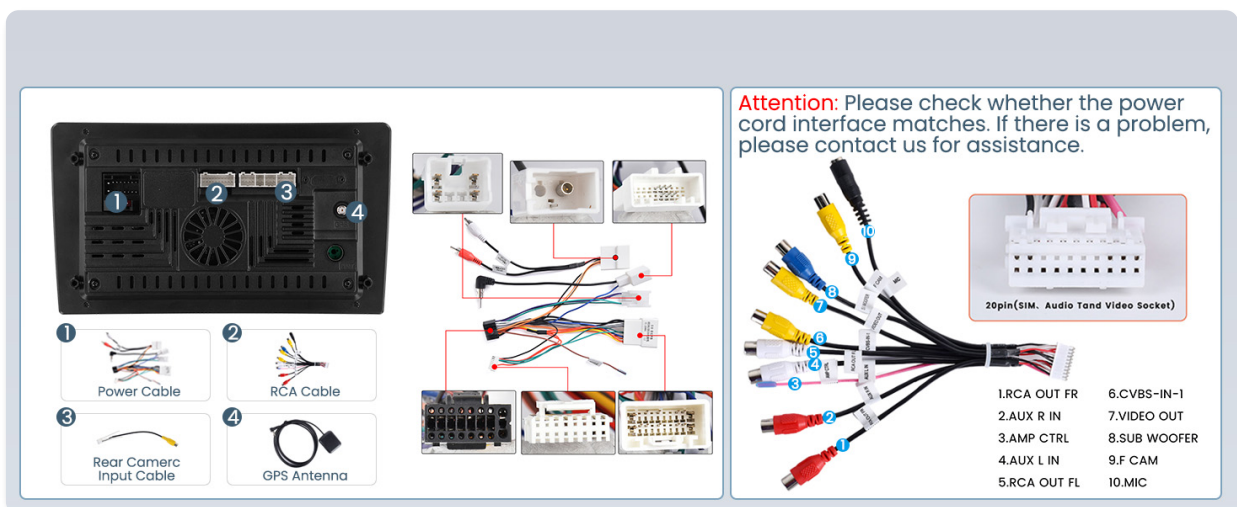
Figure 4: Port Details and Wiring Diagram. This image illustrates the various ports on the back of the car radio and provides a detailed wiring diagram for connecting the power cable, RCA harnesses, and other components.
