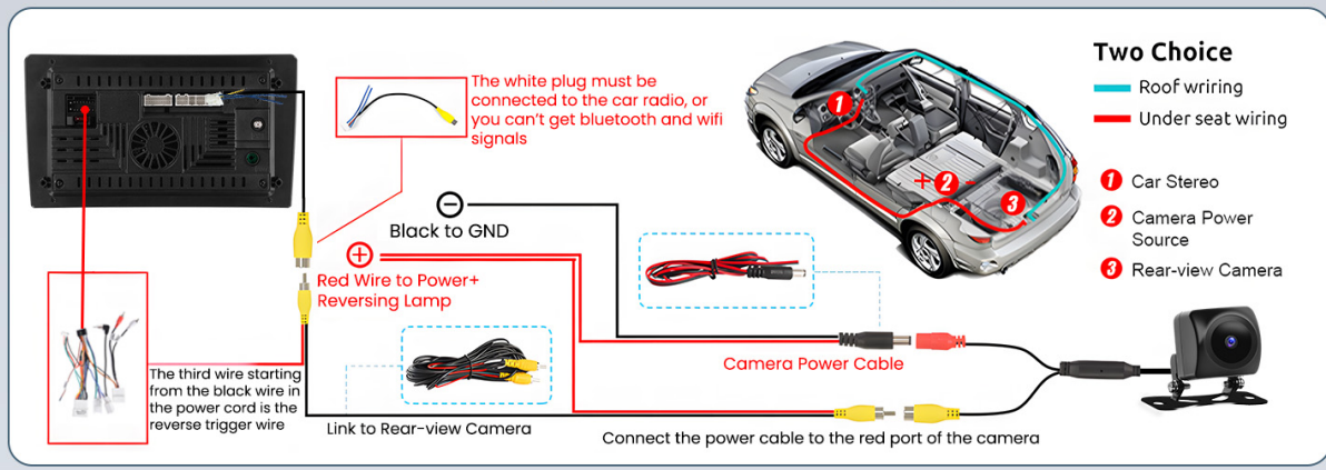
Figure 5: Backup Camera Wiring. This diagram shows how to connect the backup camera, including routing the cable through the vehicle and connecting it to the reverse light's positive pole and the car radio.
