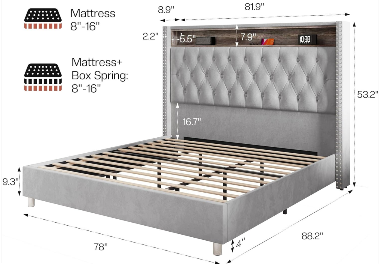
Image 4.1: An illustration showing the overall dimensions and key structural components of the King size bed frame, including the headboard, side rails, footboard, and slat system.
