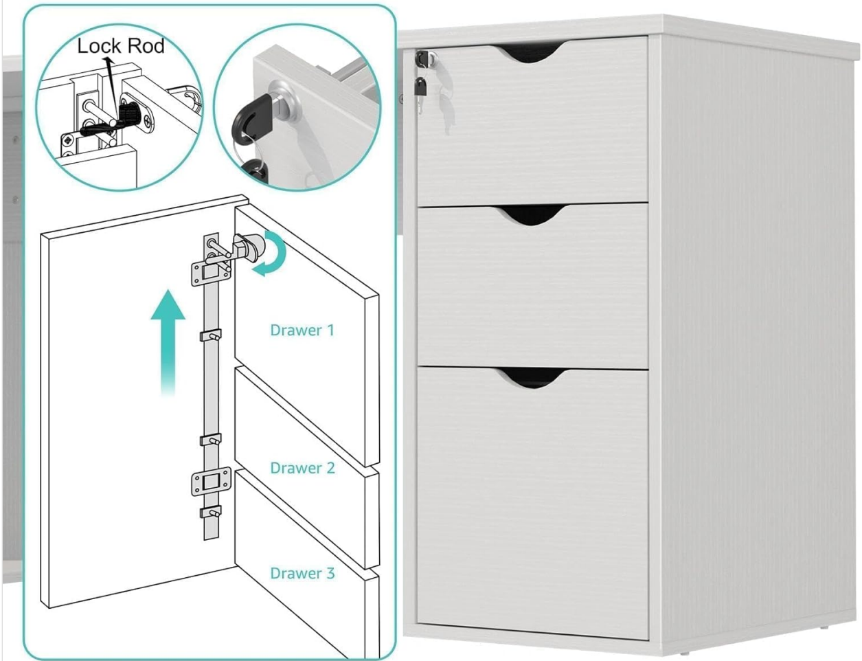
Figure 4: Illustration of the secure multi-drawer interlock system.
