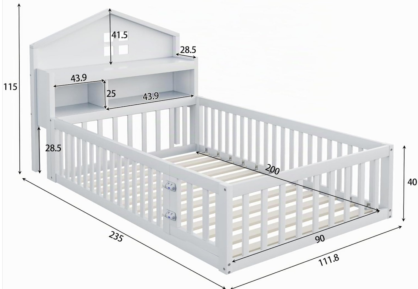
Figure 1: Overall dimensions of the Merax Children's Cabin Bed (235L x 111.8W x 115H cm).
