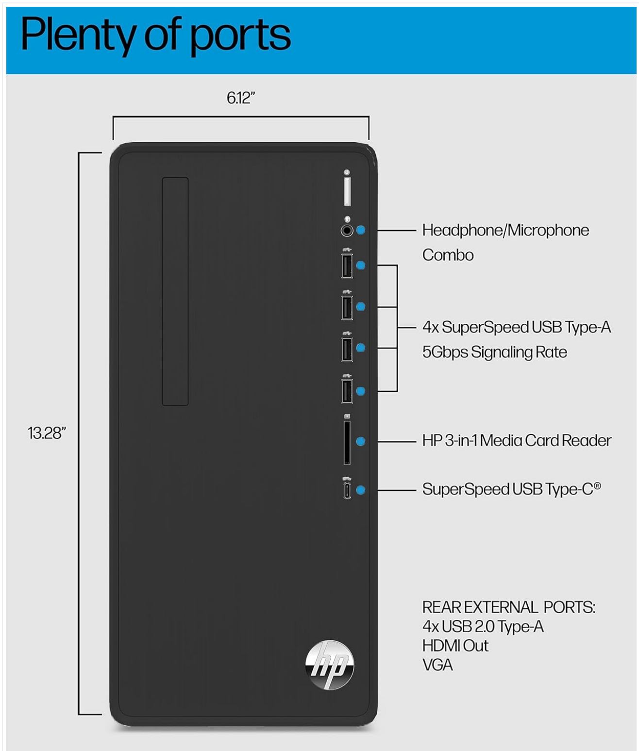
Figure 4: Rear I/O Ports for essential connections.
