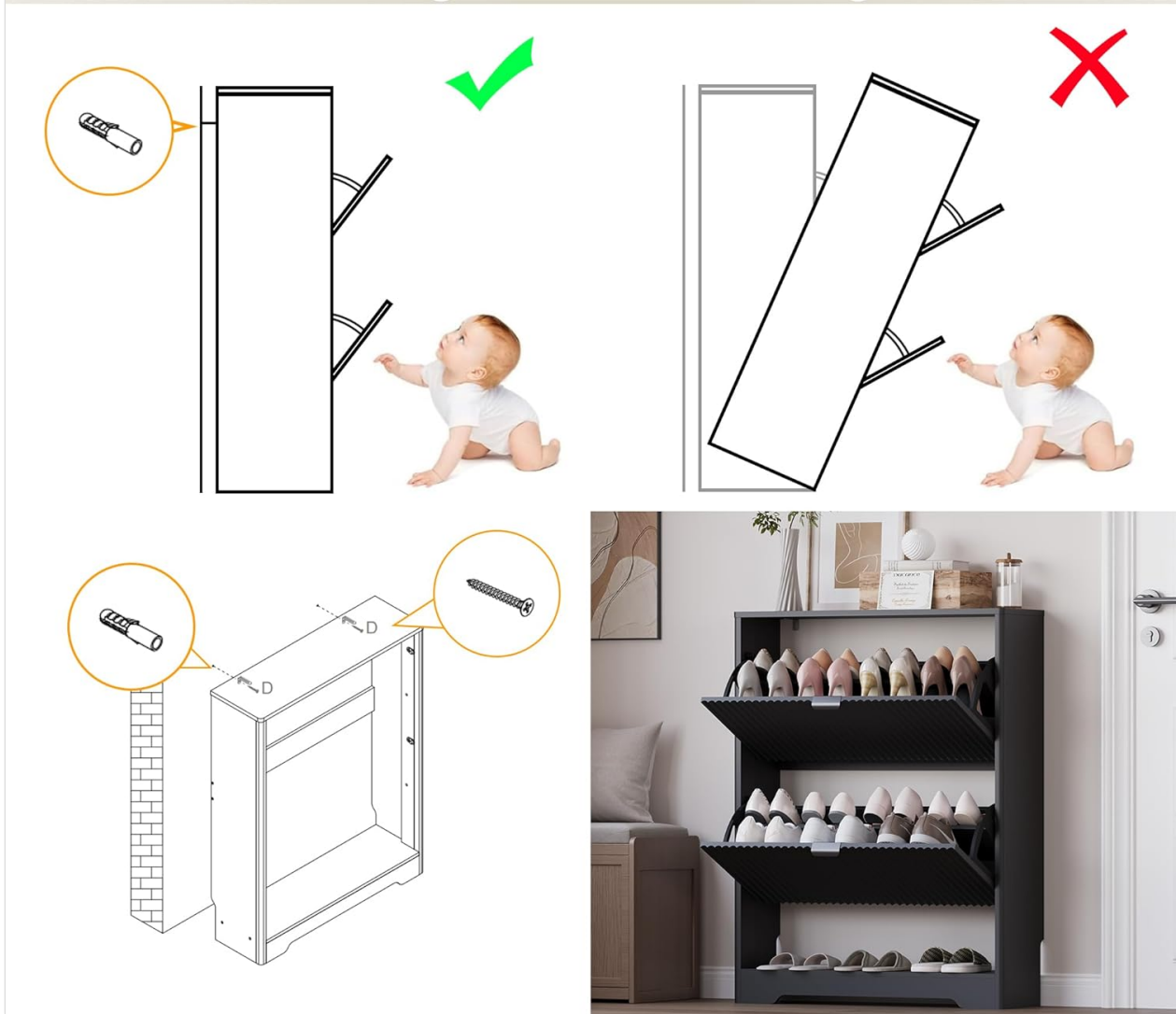
Image: Illustration of the anti-tipping wall device installation, demonstrating correct and incorrect usage to ensure stability and safety, particularly for households with children.
