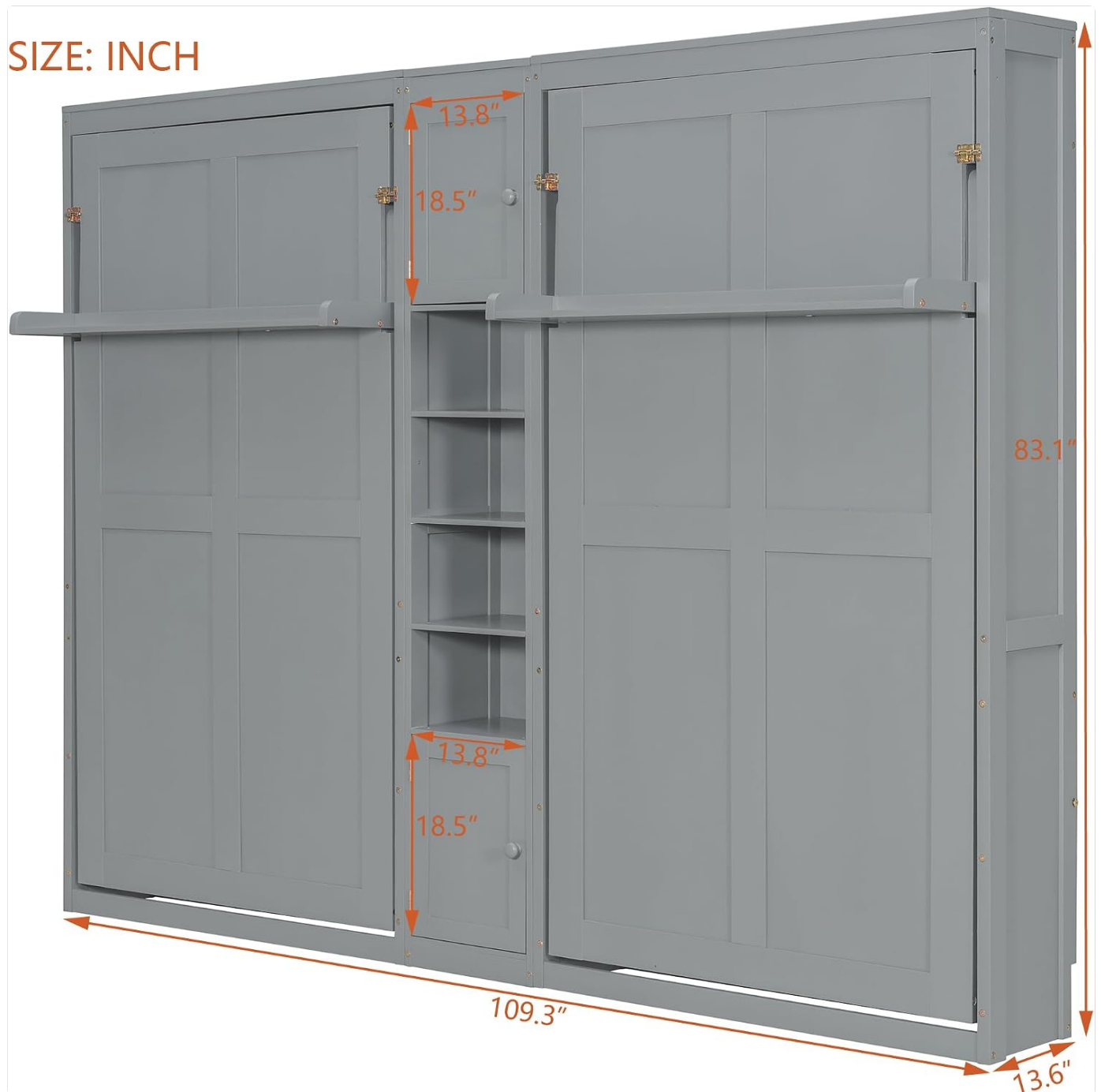
Figure 8.1: Dimensional drawing of the Murphy bed unit, showing overall and component measurements.
