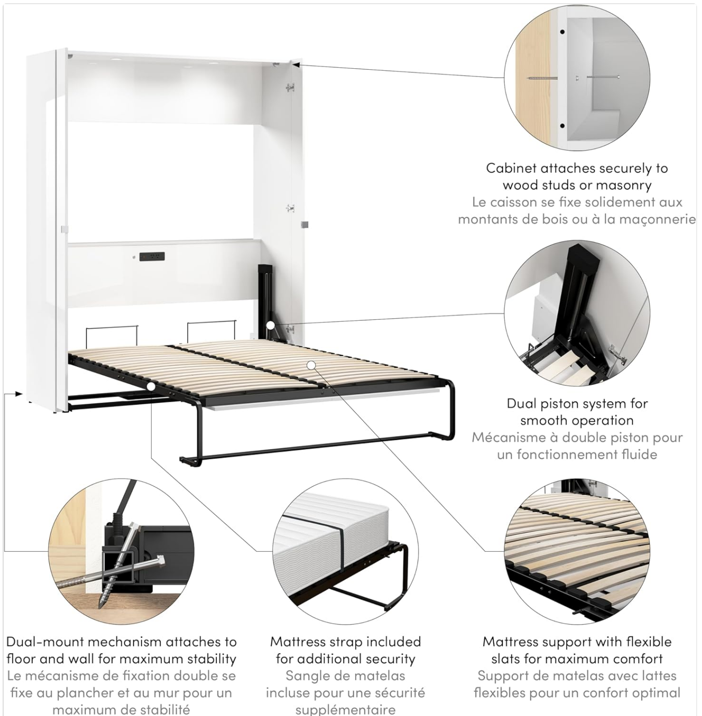
Image: A detailed diagram showing the key structural components of the Murphy bed, including the dual-mount mechanism, dual piston system for smooth operation, and flexible slat mattress support.
