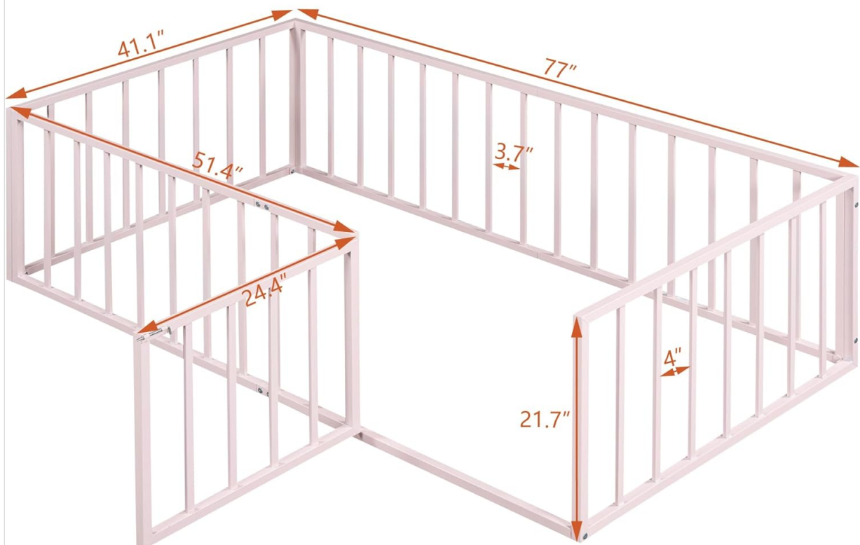
Image: A diagram showing the key dimensions of the MERITLINE Twin Floor Bed Frame in inches. It illustrates the overall length (77"), width (41.1"), and height (21.7"), along with specific measurements for the door and fence sections.
