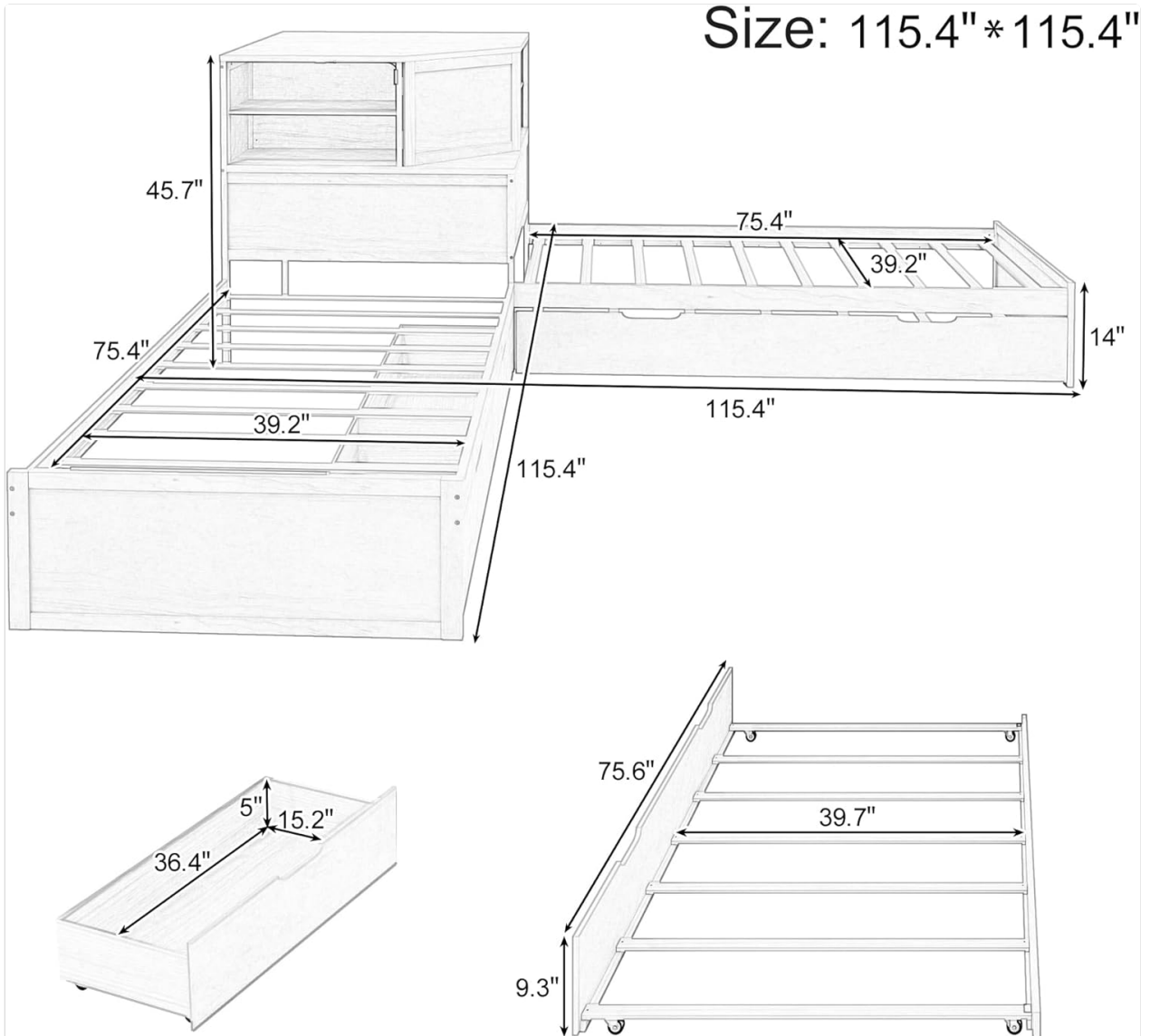
Figure 2.1: Detailed dimensions and component layout for assembly planning.
