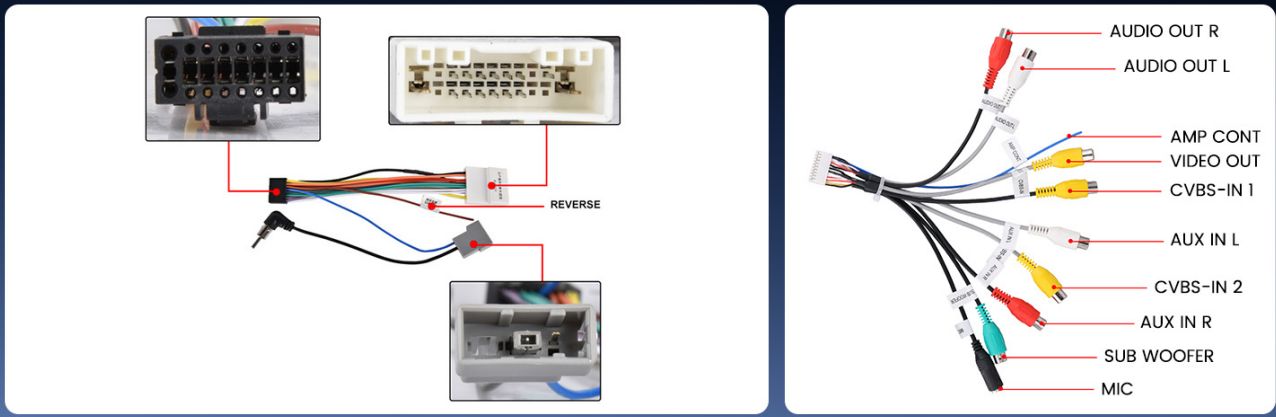
Figure 4.2: Main wiring connections for the car radio unit.
