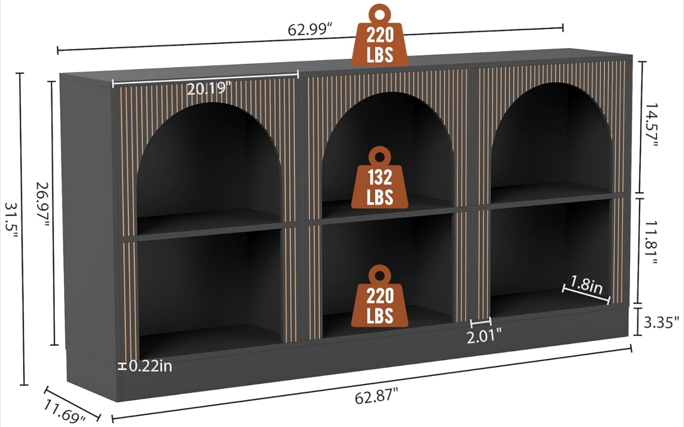
Image: Detailed diagram showing the dimensions of the console table (62.99" W x 31.5" H x 11.69" D) and weight capacities for the top (220 lbs), middle shelf (132 lbs), and bottom shelf (220 lbs).
