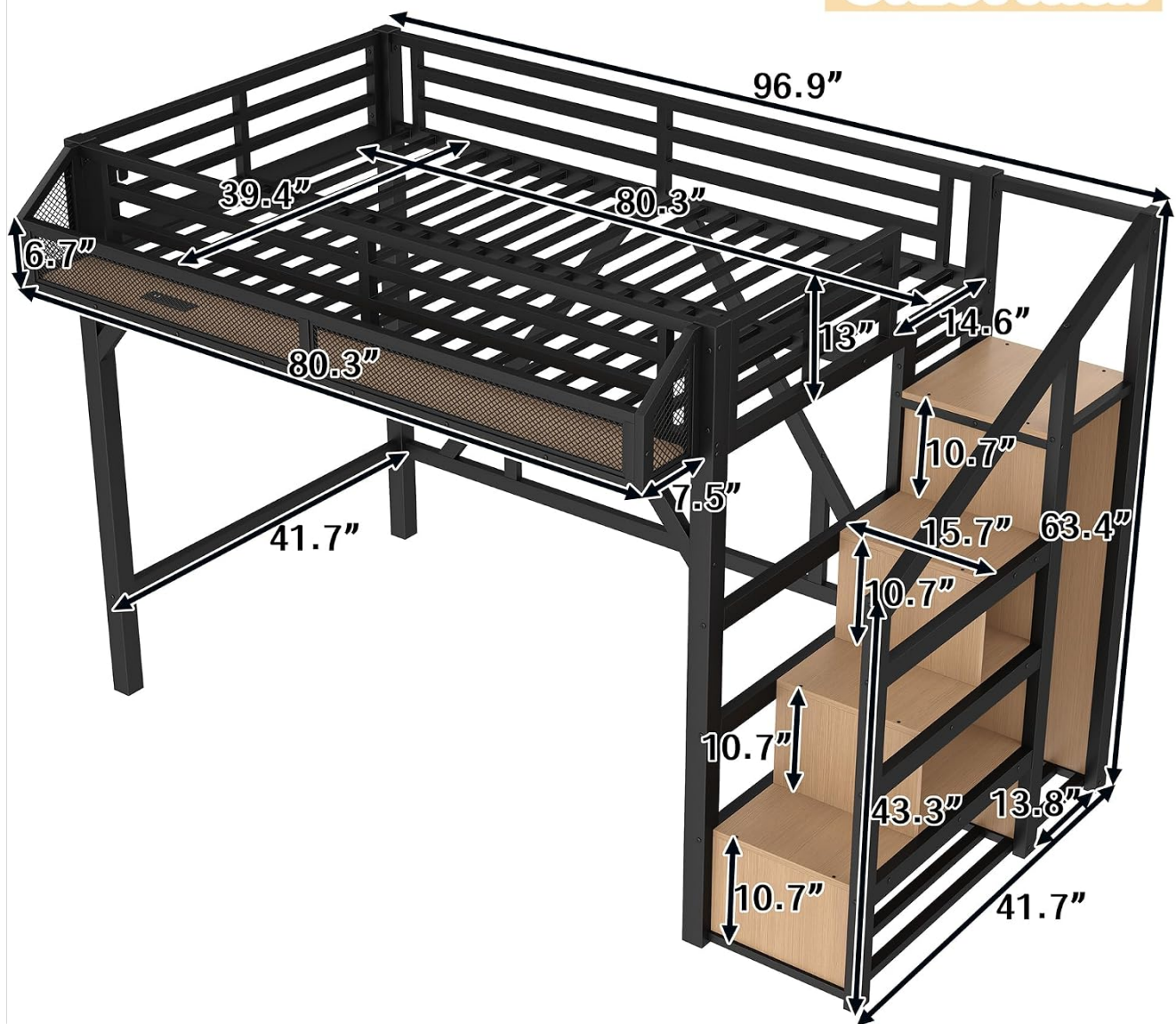
Figure 2: Product Dimensions and Structure Overview
