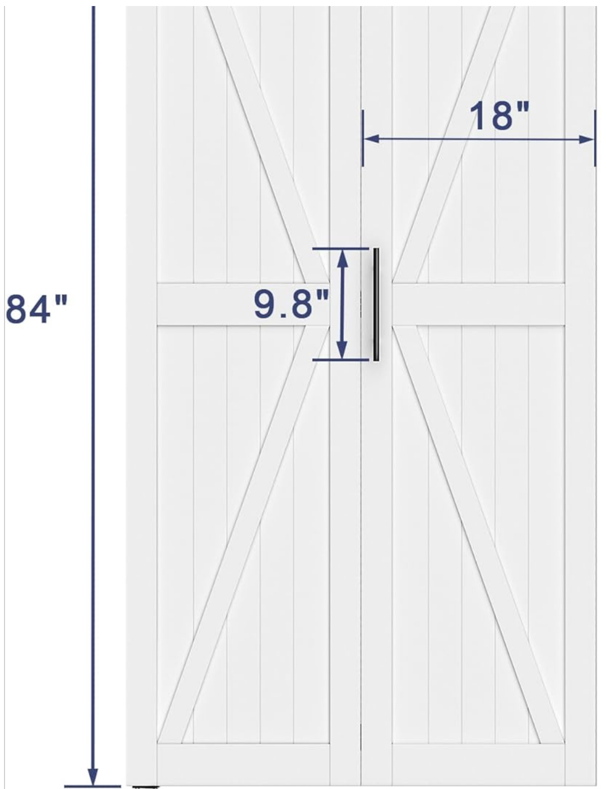
Image 1.2: Diagram illustrating the dimensions of the bi-fold door, showing a total width of 39.6 inches (including track), a height of 84 inches, and individual panel width of 18 inches.
