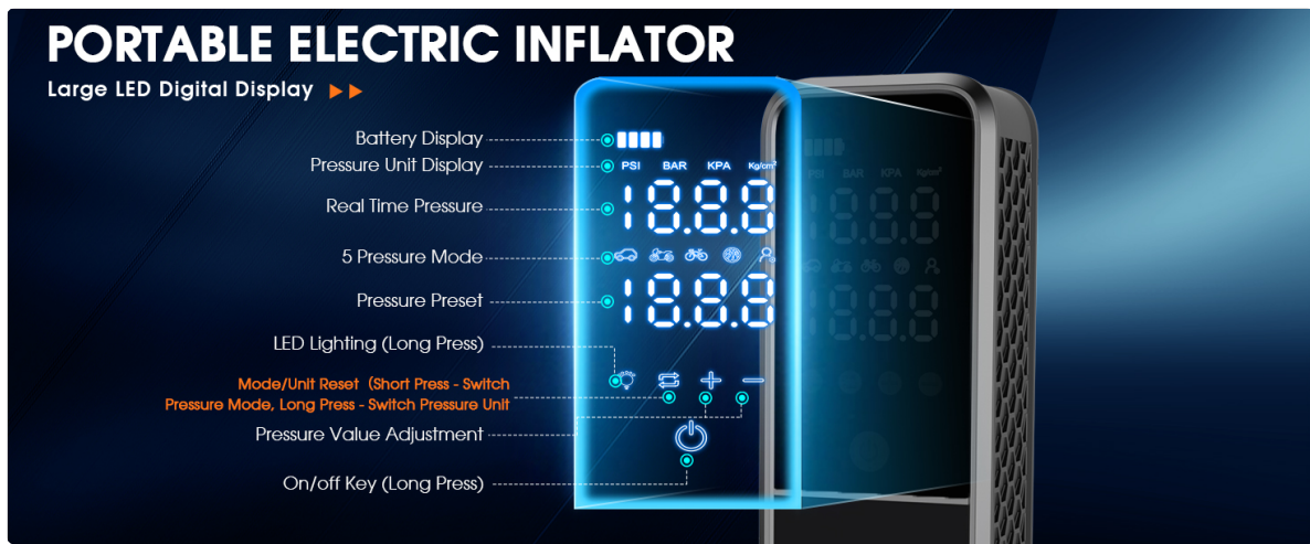
Figure 3.2: Detailed breakdown of the inflator's large LED digital display and controls. This includes indicators for battery level, selected pressure unit, real-time pressure, active pressure mode, and the preset target pressure. It also highlights the functions of the LED lighting button, mode/unit reset button, pressure adjustment buttons, and the power on/off key.
