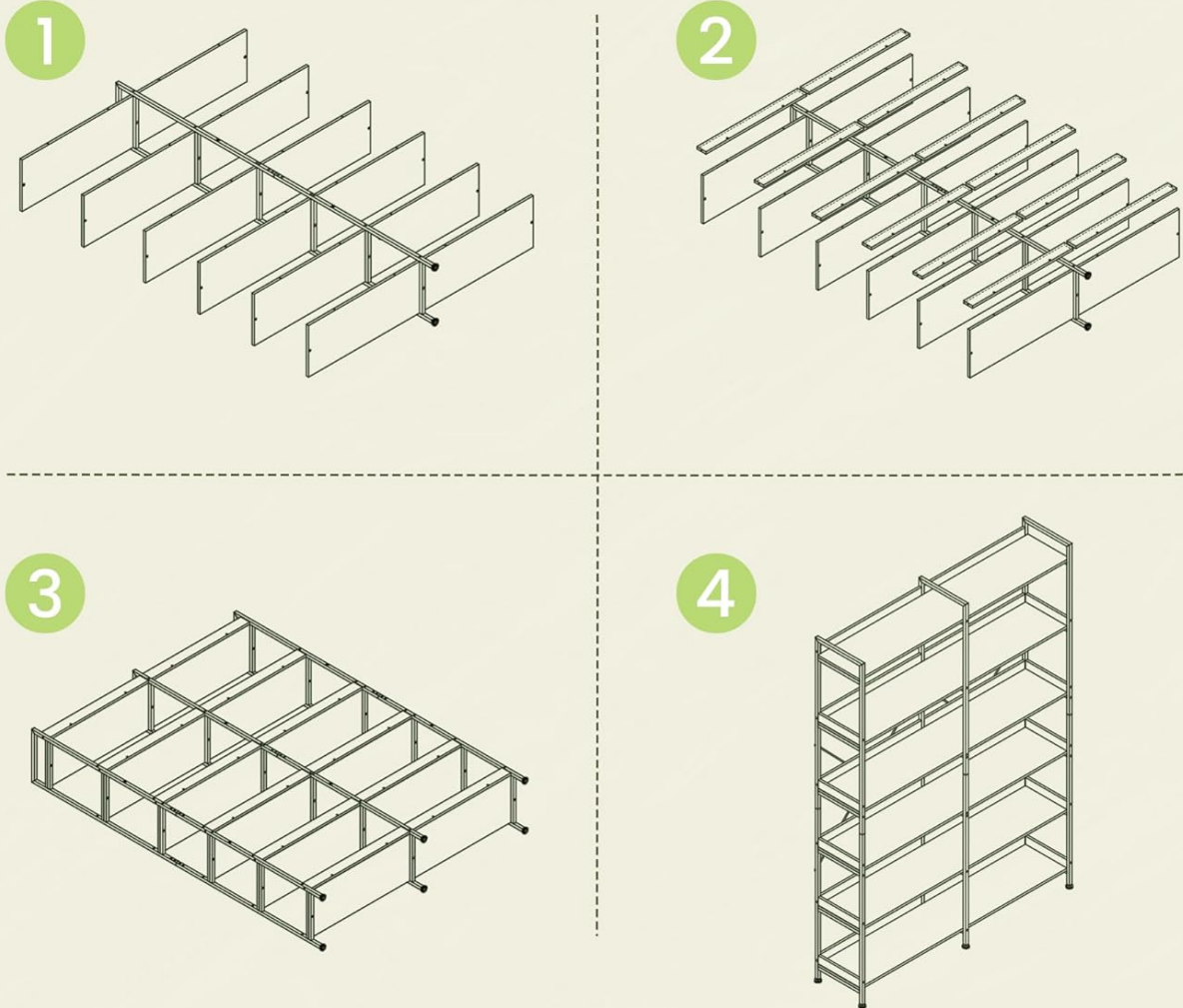
Figure 3.2.1: Visual guide for the easy installation process of the bookshelf.
