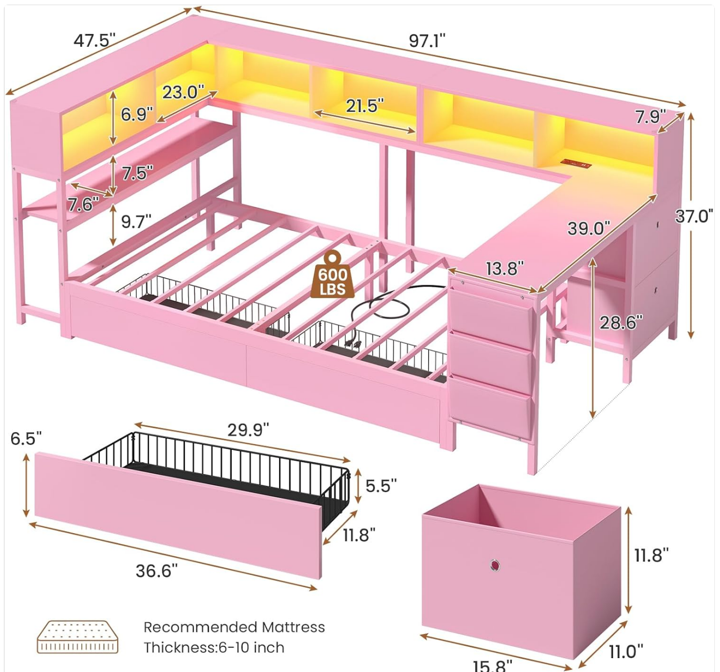
Image 8.1: Detailed dimensions of the Hasuit Twin Corner Bed frame and its components.
