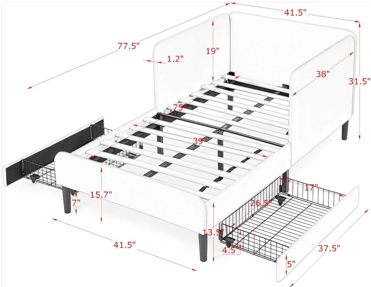
Figure 1: Product Dimensions and Component Overview. This diagram illustrates the overall dimensions of the sofa bed and highlights key structural components like the frame, slats, and integrated storage drawers.
