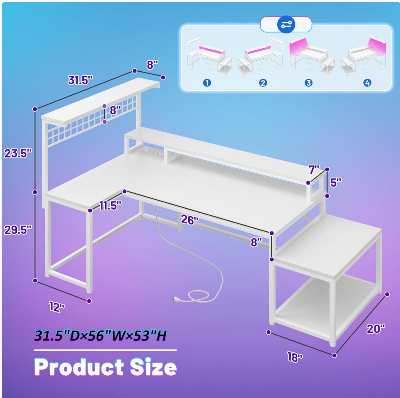
Image: An illustration detailing the dimensions of the DurayLoly L-Shaped Gaming Desk, including depth, width, and height measurements for various sections.
