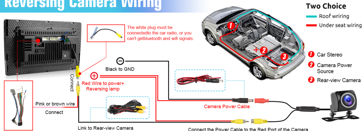
Figure 2.3: Reversing camera wiring diagram, illustrating connections for proper functionality.
