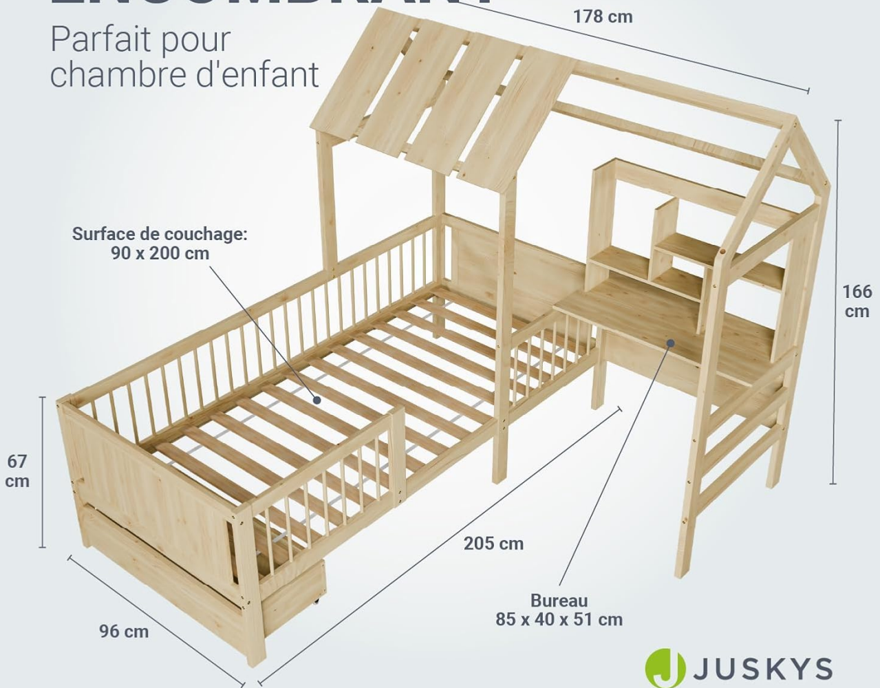
Image 3.2: A detailed diagram showing the dimensions of the Juskys Yari children's bed, including the bed frame, sleeping surface, desk, and overall height. This helps in understanding the space requirements.
