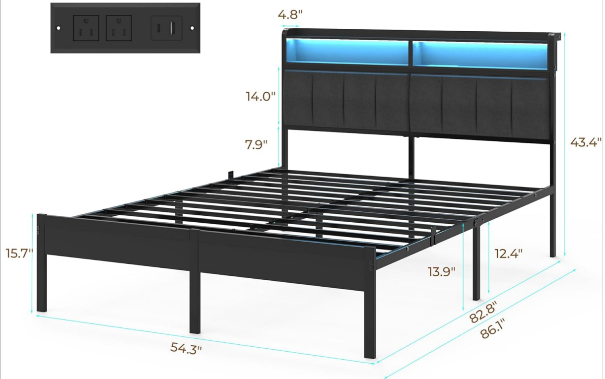
Figure 5: Dimensional specifications of the bed frame.
