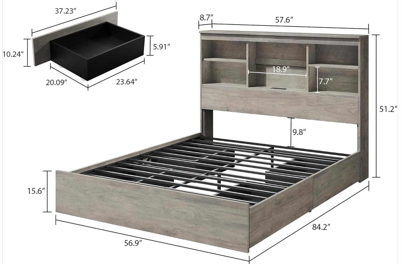
Figure 1: Overall dimensions and key components of the bed frame. Dimensions are 84.2"L x 56.9"W x 51.2"H.
