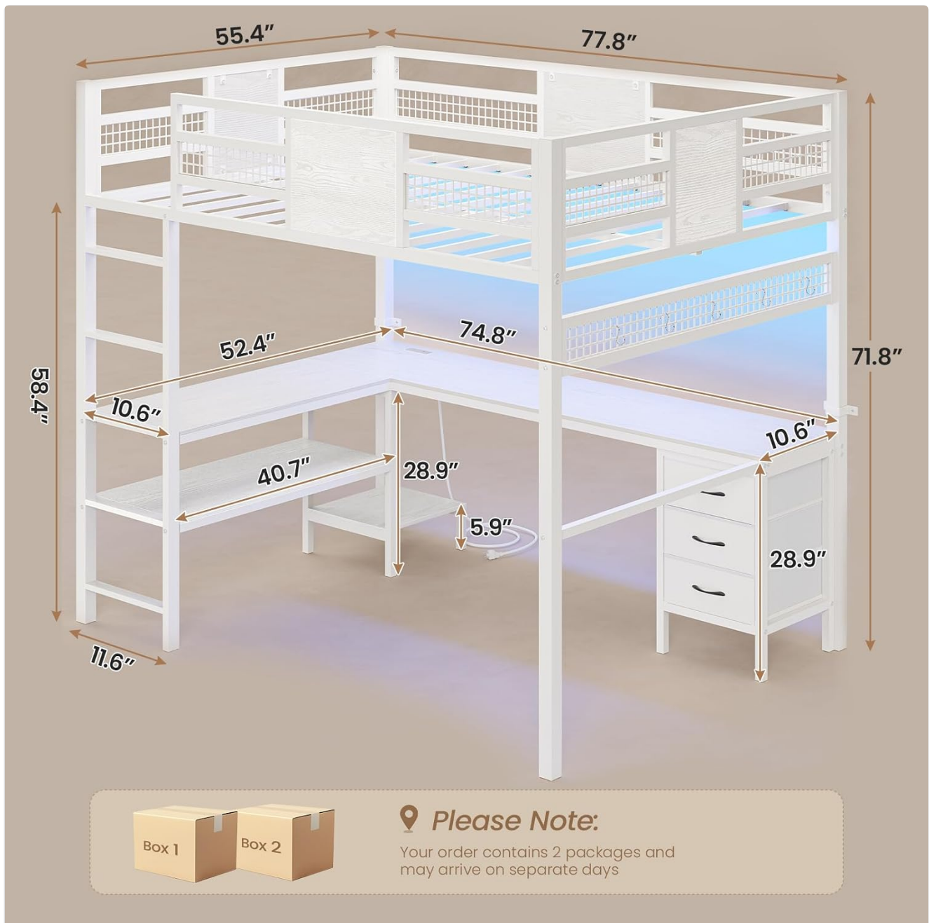
Image 4.1: Detailed dimensions of the loft bed, including height, width, and desk measurements.
