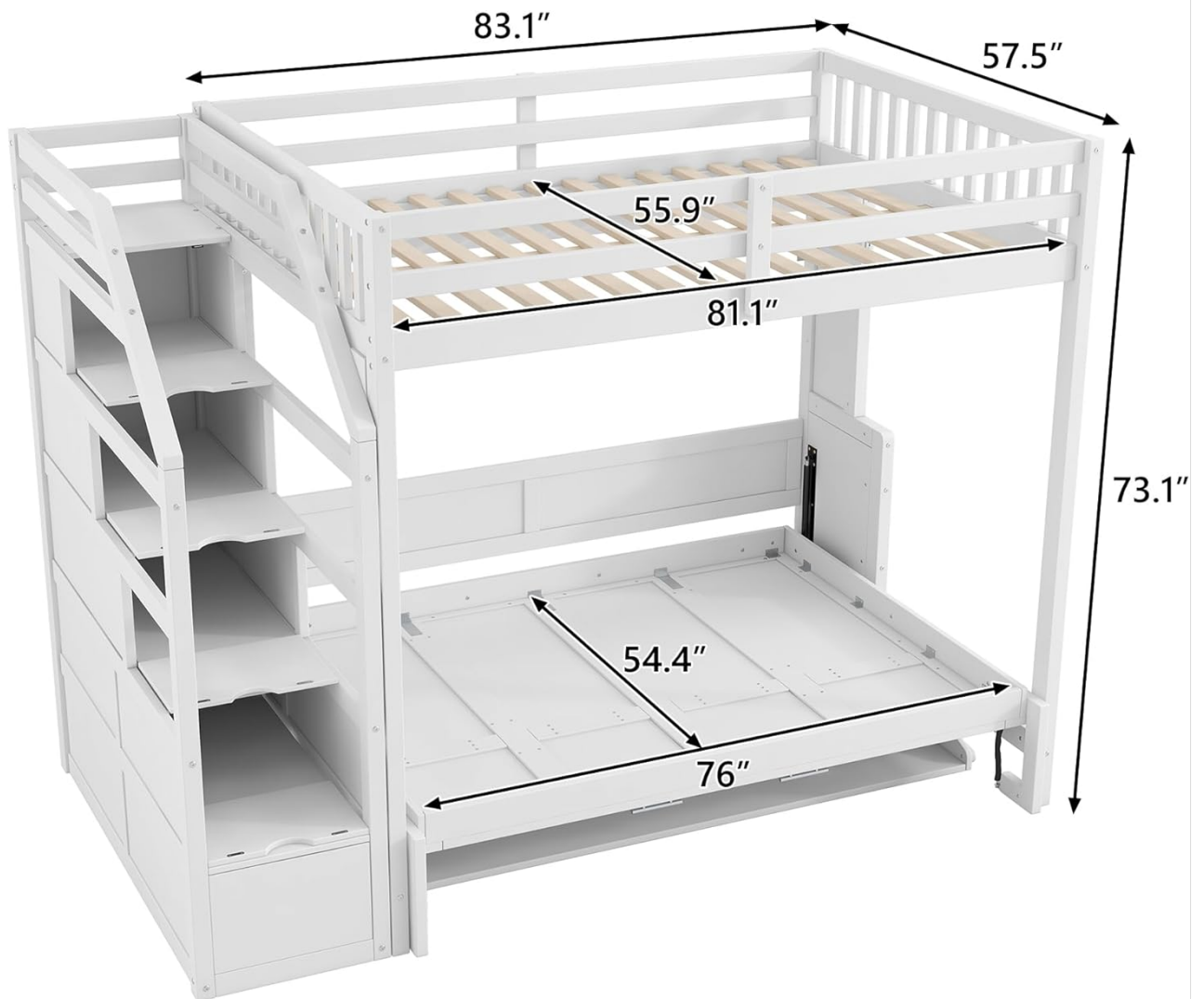
Figure 6: Detailed dimensions of the LUMISOL Full XL Loft Bed.
