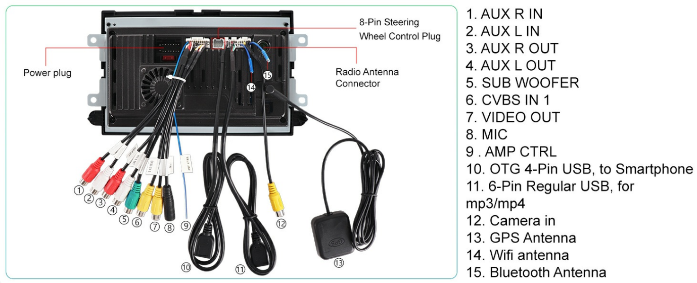
Image: A comprehensive wiring diagram showing all connection points for the ASURE Car Stereo, including power, audio, video, USB, GPS, and antenna connections.
