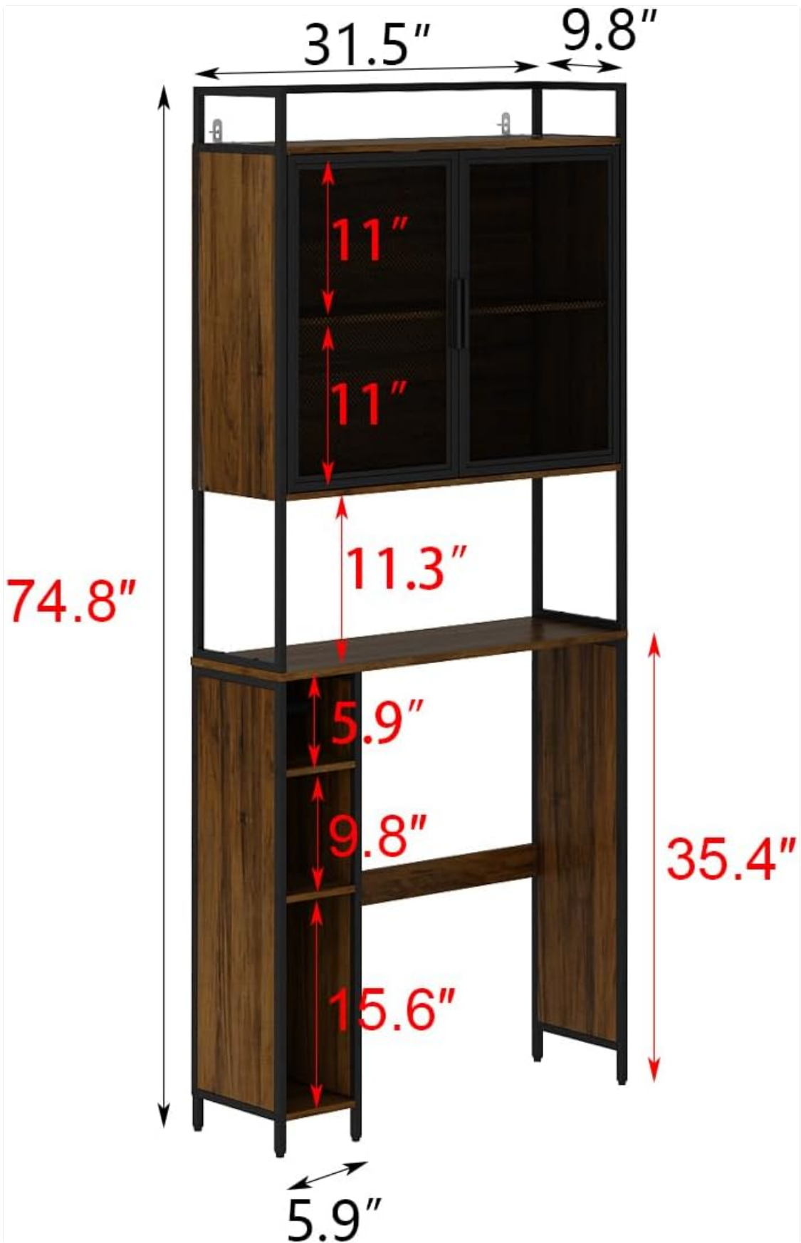
Figure 5: Detailed dimensions of the storage cabinet.
