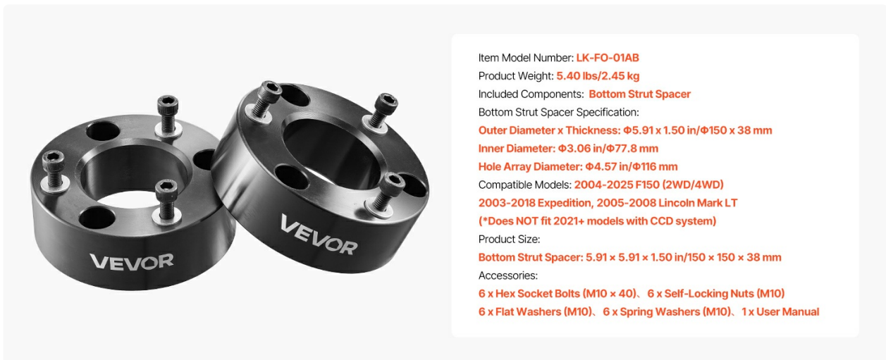
Image 4: Detailed view of the kit's components, including two strut spacers with their dimensions, and a comprehensive list of all hardware and compatible vehicle models.
