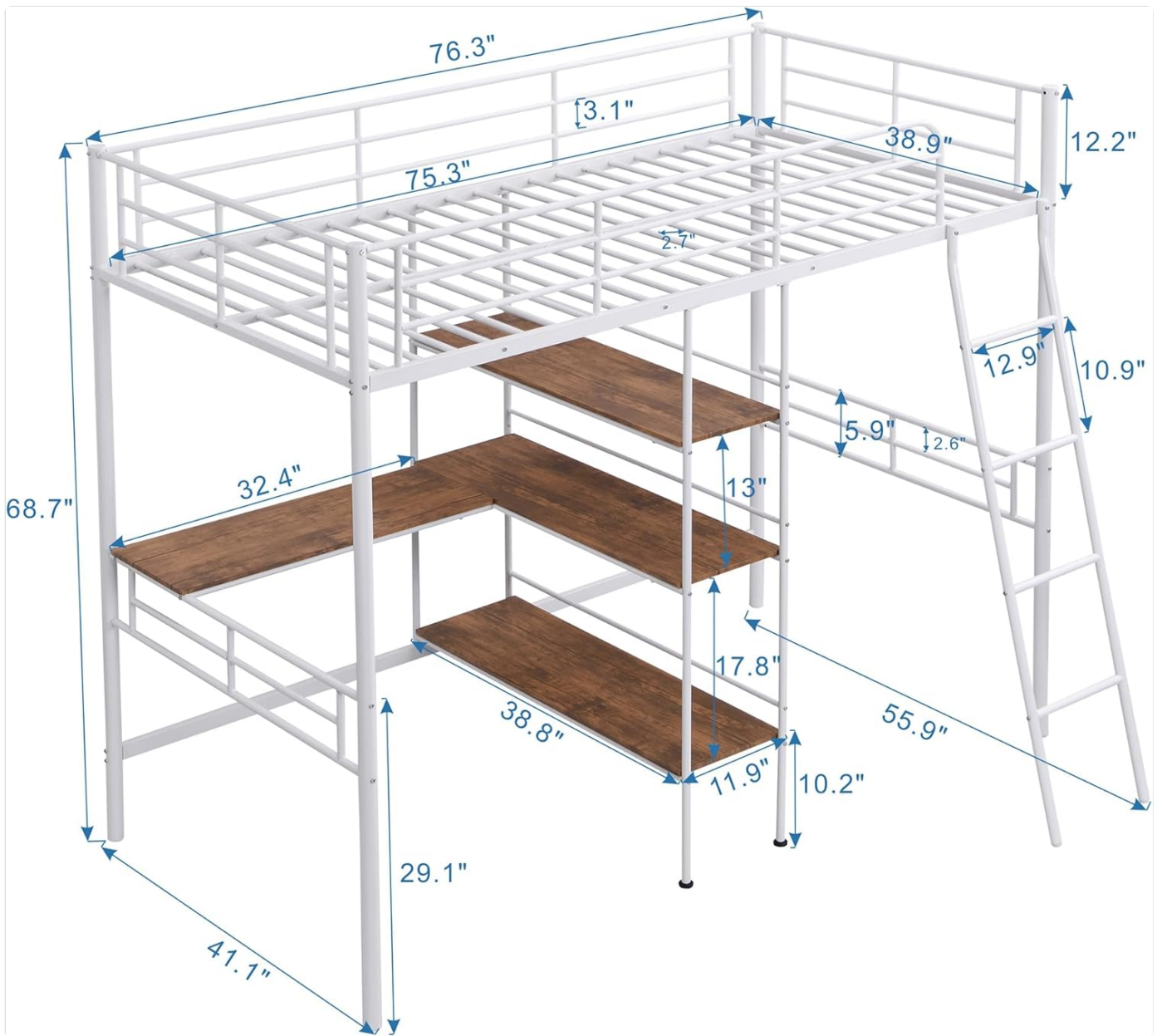
Figure 3: Detailed dimensional diagram of the loft bed, including measurements for the bed frame, desk, and shelves. This diagram is helpful for planning placement and understanding component sizes during assembly.
