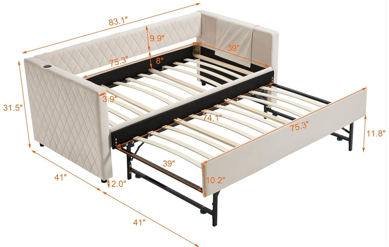
Image: A technical diagram illustrating the precise dimensions of the SOFTSEA Twin Daybed, including length, width, height, and internal measurements for both the main bed and the trundle.
