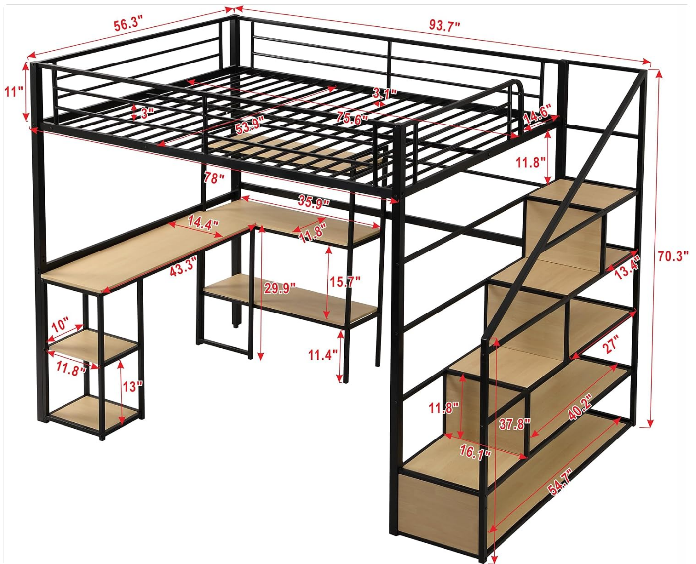
Image: Detailed diagram showing the dimensions of the loft bed, including length, width, height, and measurements for the desk and storage areas.
