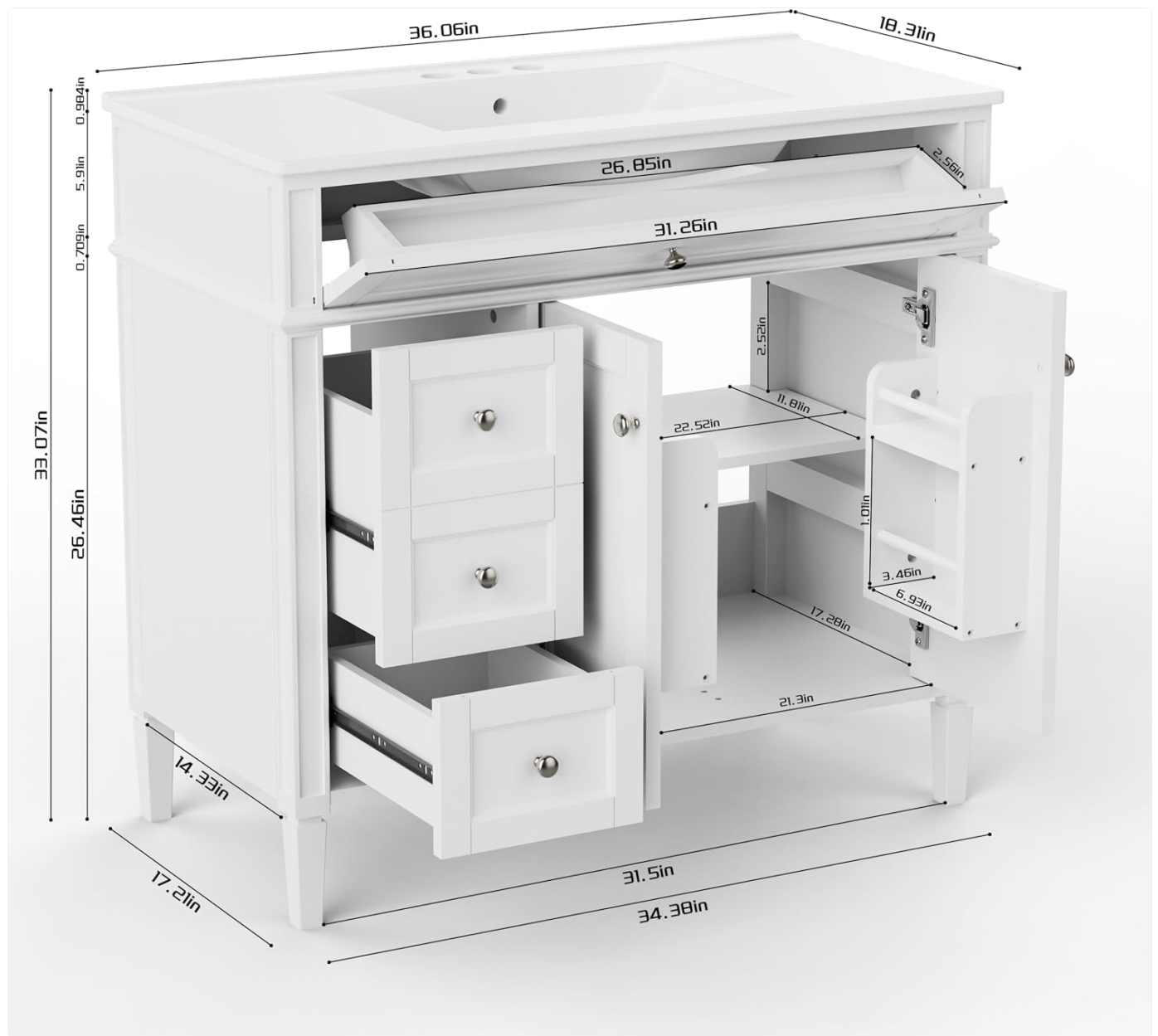
Image: Detailed dimensions of the OWIPAW 36-inch Bathroom Vanity, illustrating various measurements for installation planning.
