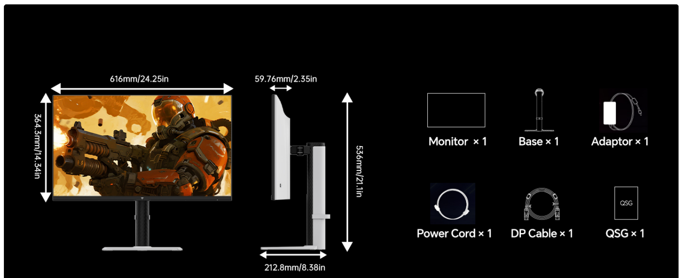
Image 2.1: Illustration of all components included in the KTC H27T6 monitor package.
