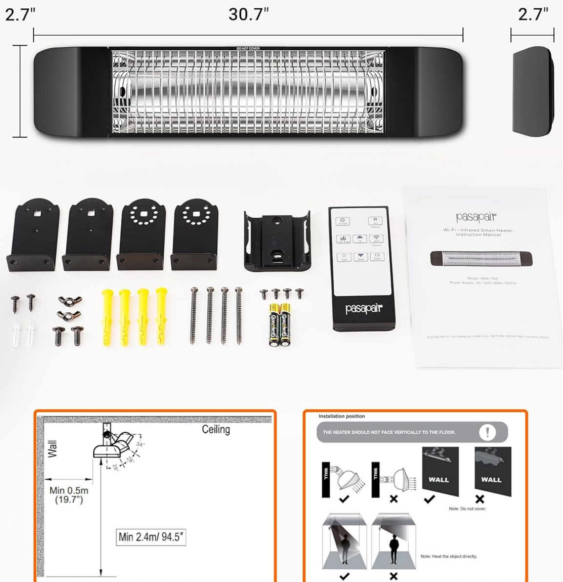
Image 3.1: Heater dimensions, included mounting hardware, and critical installation guidelines for wall placement.
