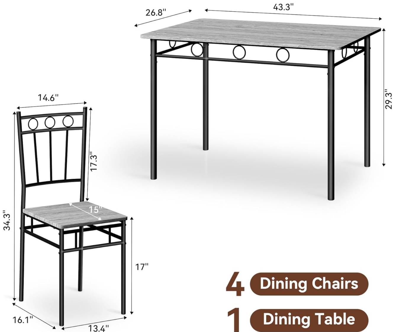
Image: Detailed dimensions of the dining table and chairs.
