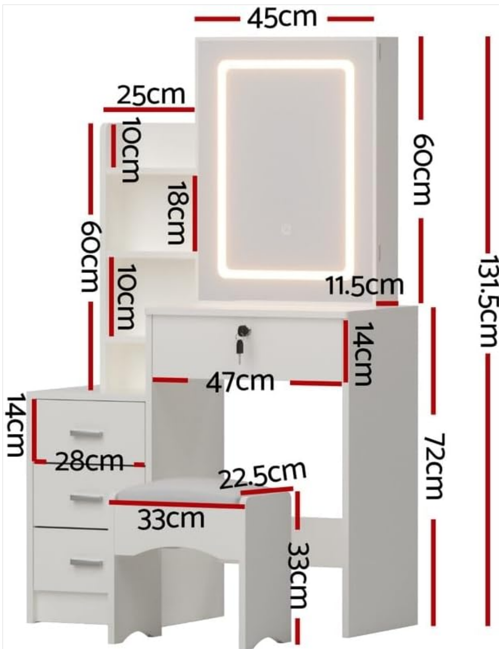
Image 4.1: Product Dimensions. This diagram provides a comprehensive view of the dressing table's dimensions in centimeters, including the overall height, width, and depth, as well as the individual measurements for the mirror, shelves, drawers, and stool.
