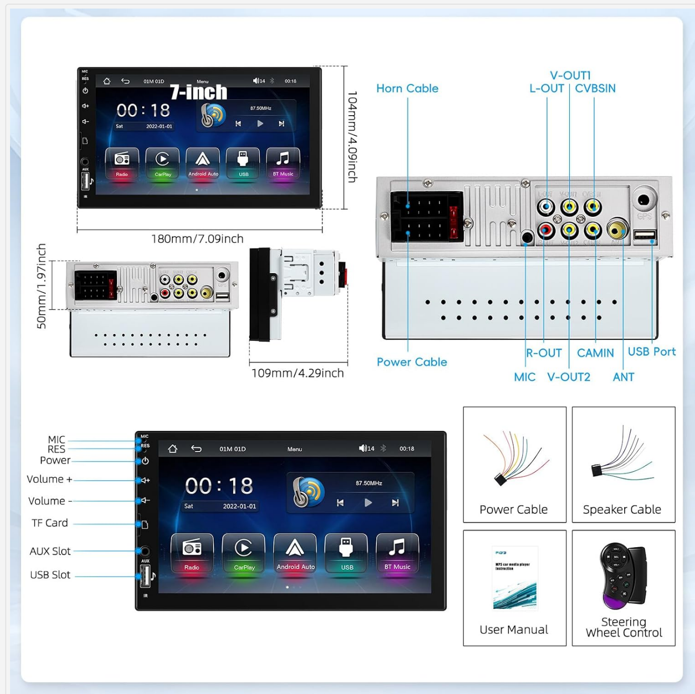
Figure 3.1: Main unit dimensions, rear connections, and included accessories.
