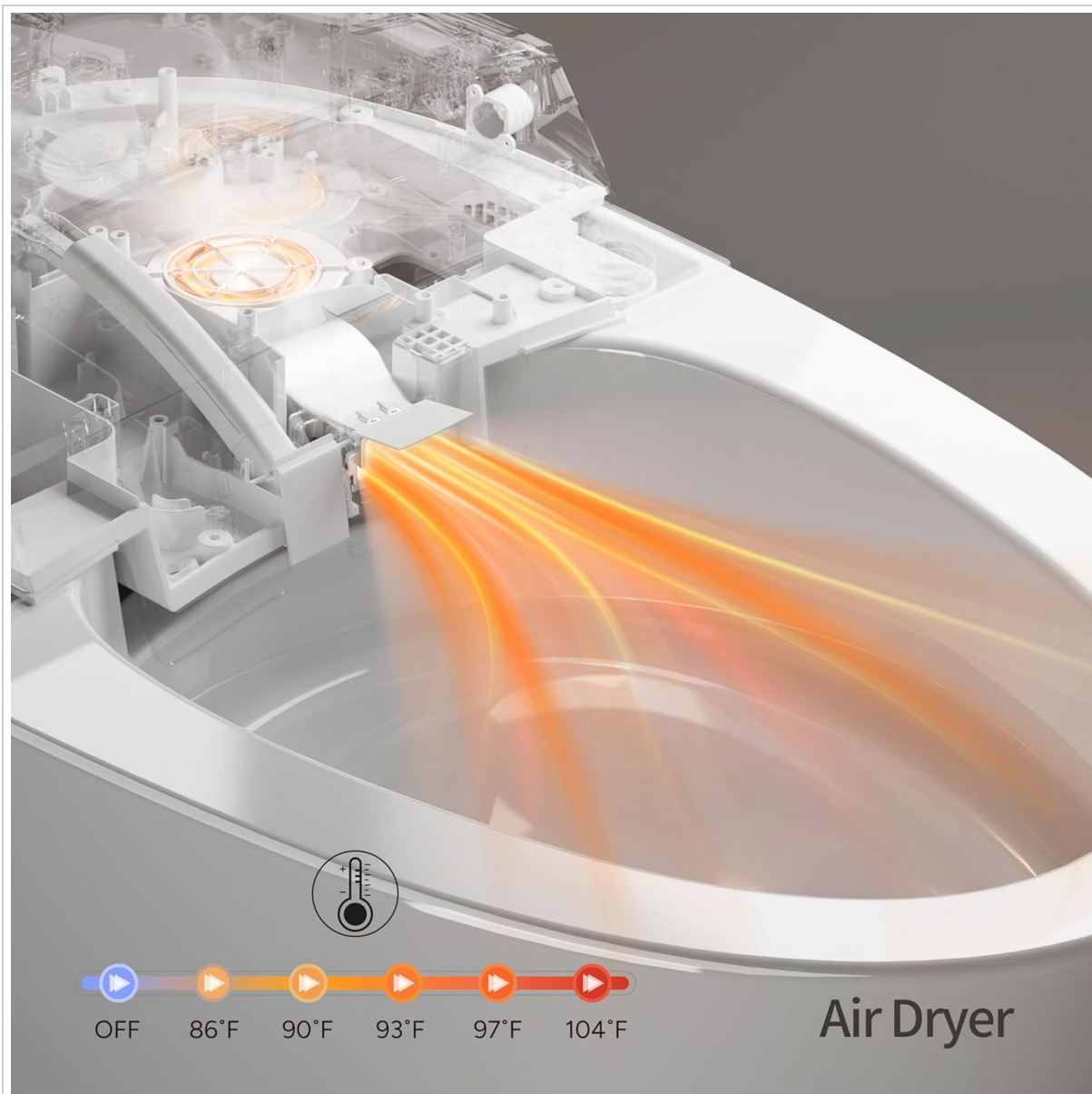
Figure 6: Warm air dryer mechanism and temperature options.
