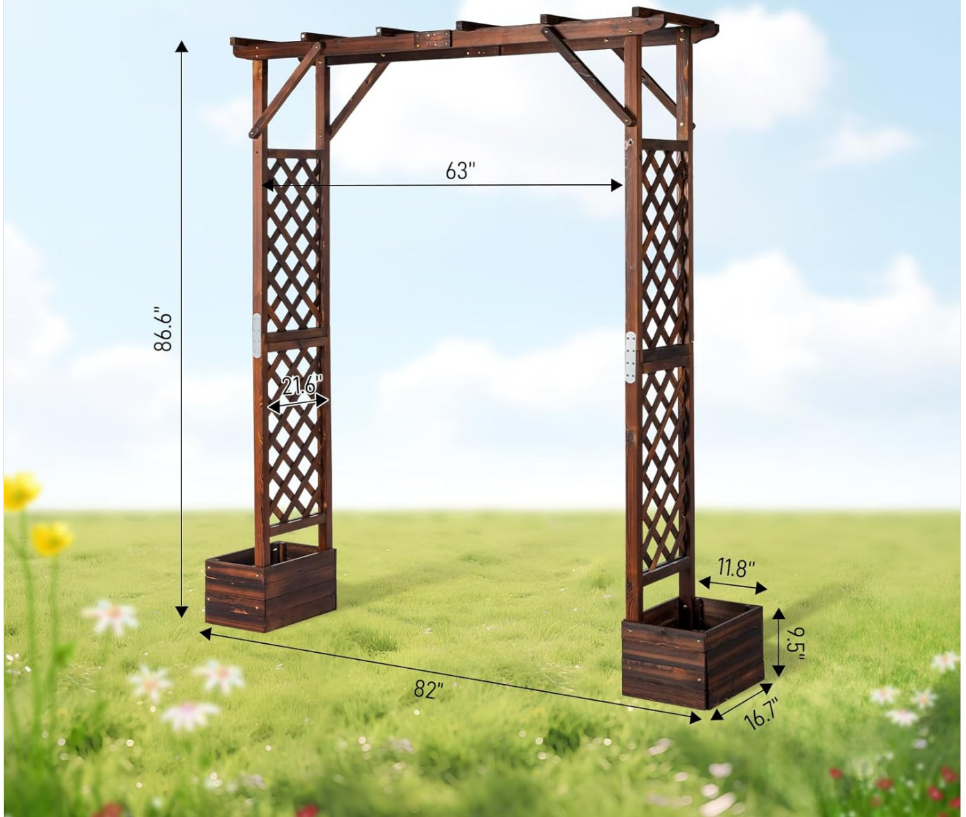
Image 4.1: Product dimensions for planning placement and assembly. Dimensions are approximately 21.6" W x 86.6" H.
