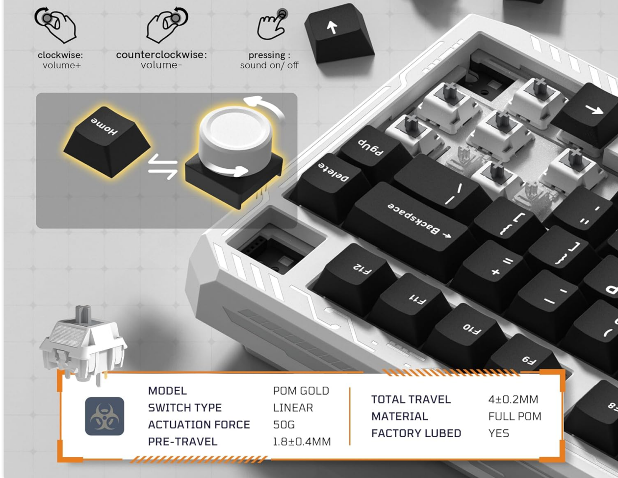
Image 5.3: Detailed view of the hot-swappable volume knob and its functions, alongside the hot-swappable switch sockets.
