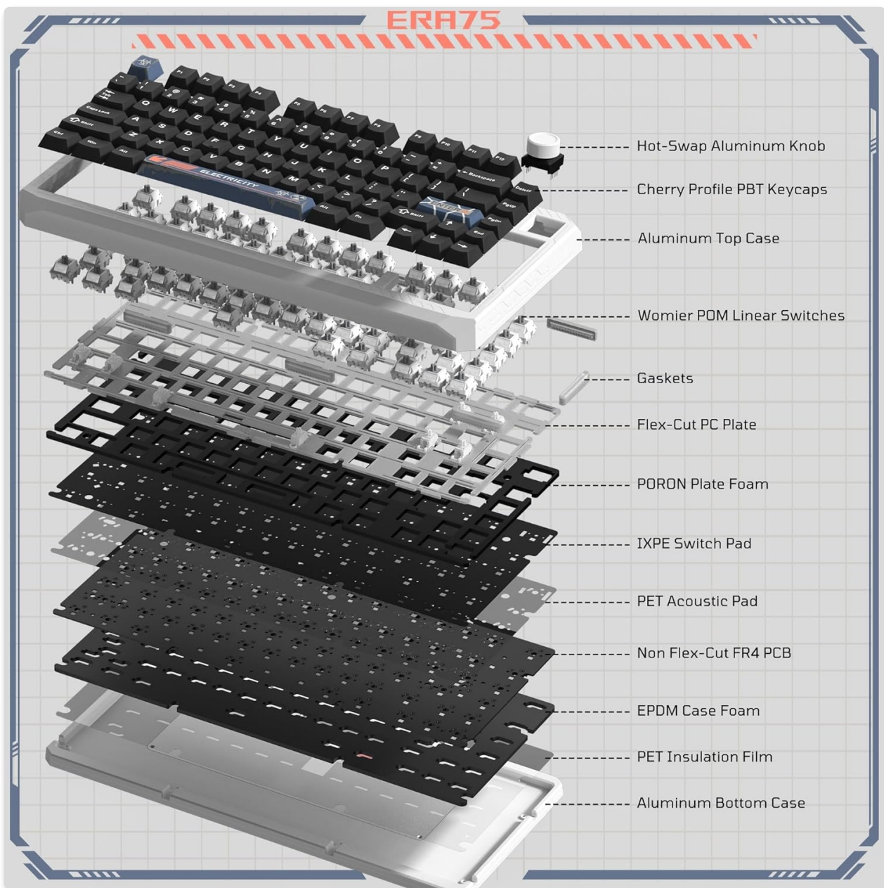
Image 8.1: Exploded view illustrating the internal layers and components of the Womier ERA75 keyboard, including the aluminum case, switches, gaskets, and PCB.
