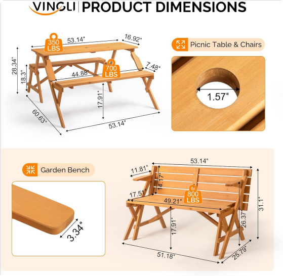
Image: Comprehensive dimensions for both the picnic table and garden bench configurations, including weight capacities.
